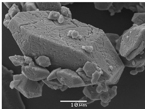
Figure 11. Scanning Electron Microscopy photograph of the \gamma -HNIW crystals, obtained by heating RS- \epsilon -HNIW for 30 minutes at 190 °C by means of isothermal TG in the sense of the method described in paper [18].
