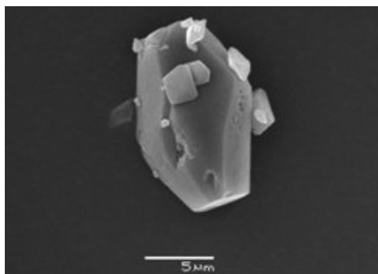
Figure 1. Scanning Electron Microscope photograph of the normal \epsilon -HNIW crystals used [11].
