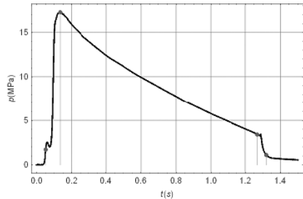
Figure 8. Dependence of p=f(t) for propellant P2.
