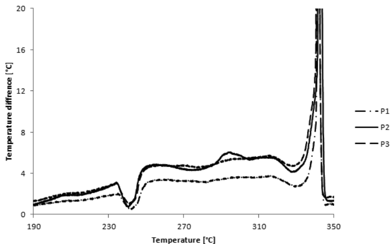
Figure 4. DTA thermograms of the propellants tested.
