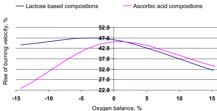
Figure 7. Influence of oxygen balance on the increase in burning velocity between 1 and 2 mm thick walls for both lactose and ascorbic acid based compositions at 1.73 g/cm 3 charge density.
