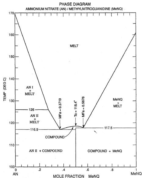
Figure 3. T-X phase diagram of the MeNQ/AN binary system reported in the literature [1].
