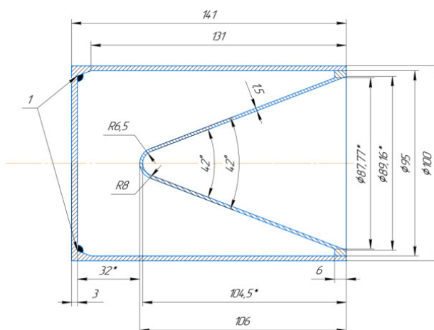
Figure 5. Scheme of an SC with a liner in the form of a cone with an angle at the top of 42^\circ and a wall thickness of 1.5 mm
